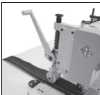
Clutch driven puller feed mechanism
